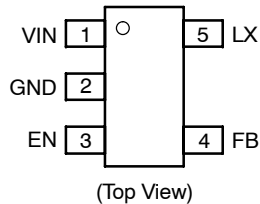
Figure 4. Pin Connections
