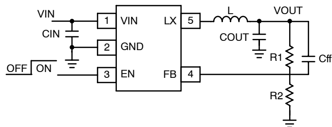
Figure 1. Typical Application
